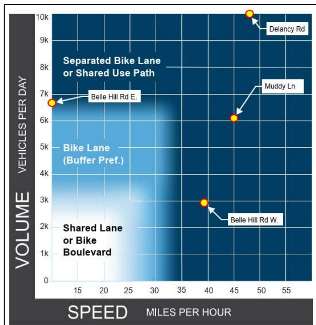
Figure 4-4: FHWA Preferred Bikeway Type for Urban, Urban Core, Suburban, and Rural Town Contexts
